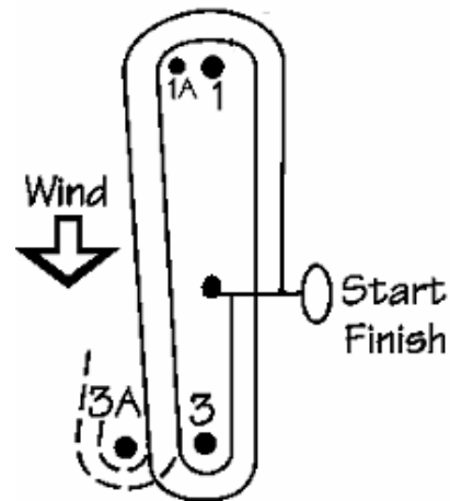
Windward-Leeward Twice Course Start - Mark 1, Mark 1(a) Offset, Mark 3 or 3a, Mark 1, Mark 1(a) Offset, Mark 3 or 3a, Finish
